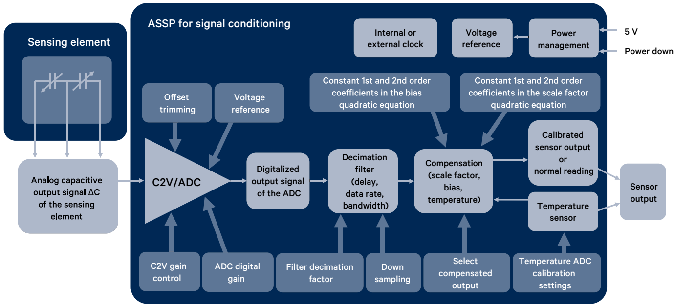
Fig. 1: Block diagram of the sensor system
