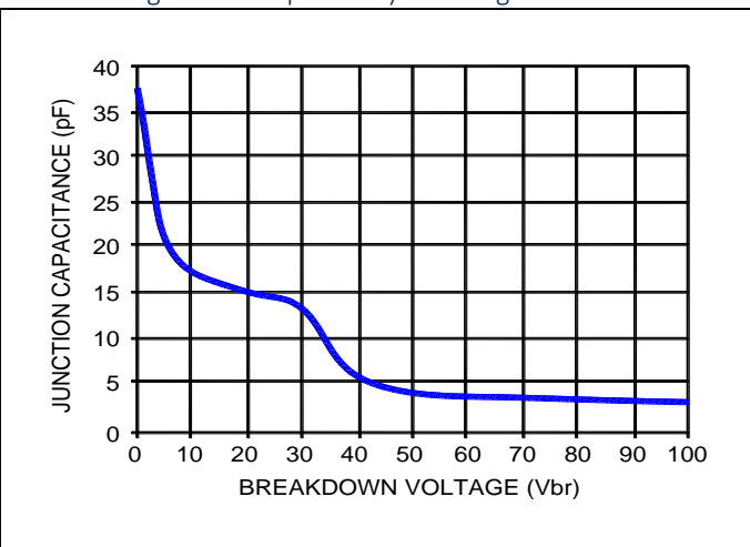
Fig.4 : APD capacitancy vs voltage
