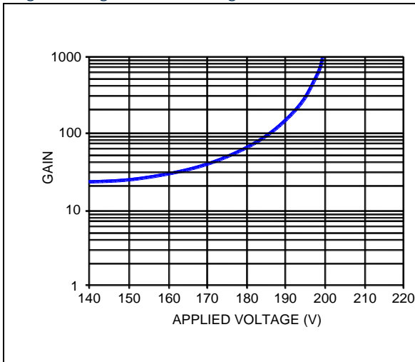
Fig. 1: APD gain vs bias voltage
