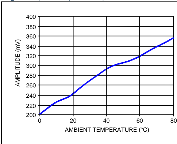
Fig. 3 : Amplifier output vs temperature
