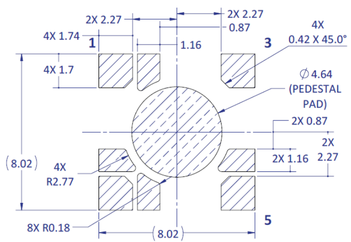
Figure 2a: Recommended solder pad layout for anode, cathode, and thermal pad for non-pedestal and pedestal design
