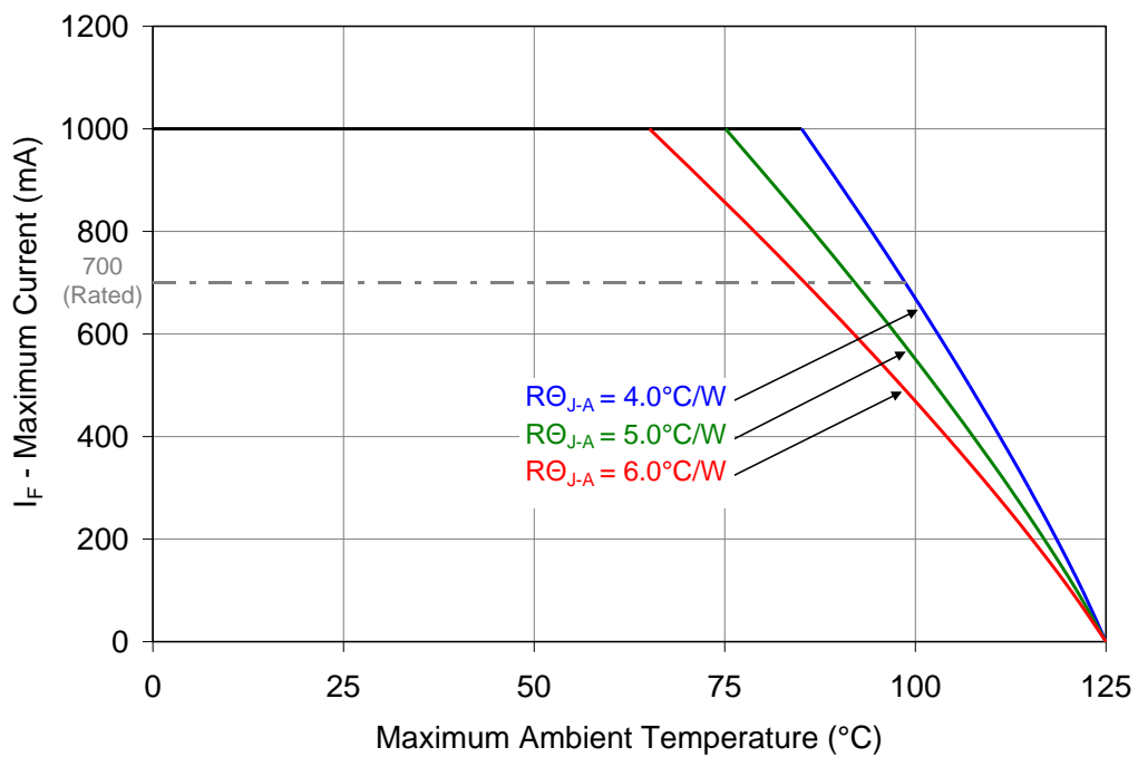
Figure 11: Maximum forward current vs. ambient temperature based on T_{J(MAX)} = 125^\circ\text{C}
