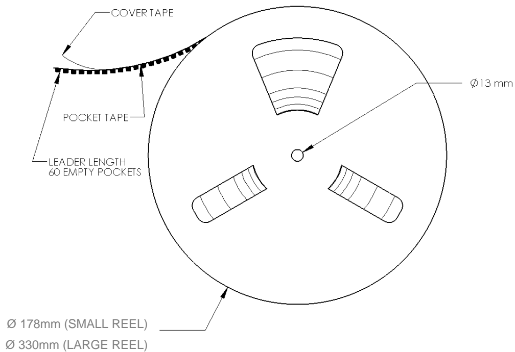
Figure 11: Emitter reel specifications (mm)
