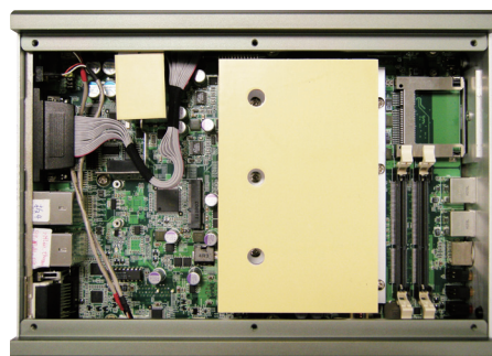
» Fanless Design
