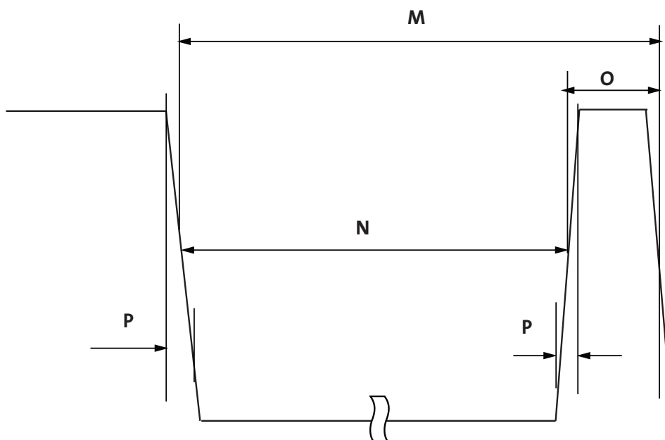
Figure 49: V Pulse
