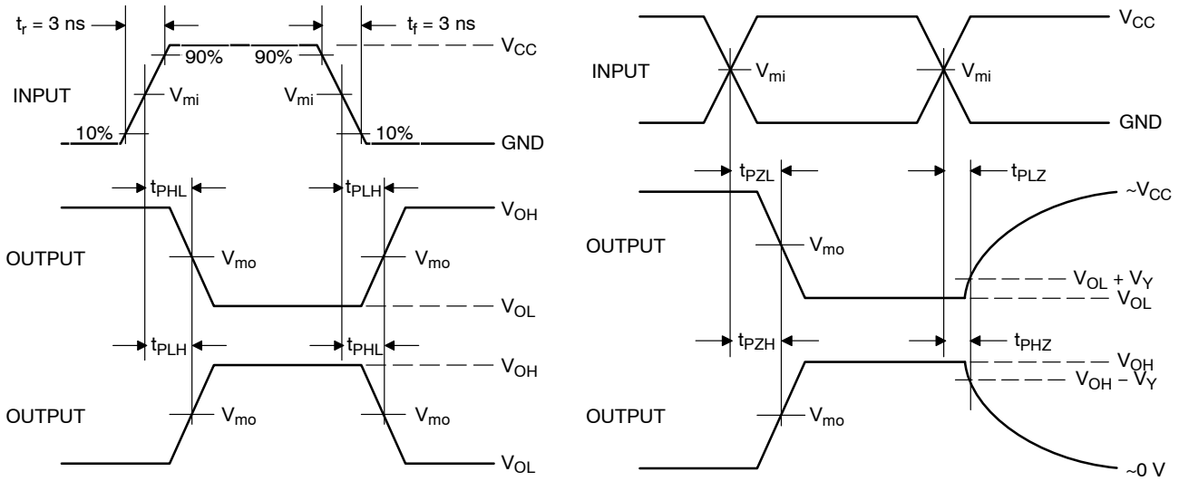
Figure 2. Switching Waveforms
