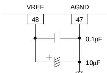
Figure 8.2 VREF External Circuit Connection Diagram
