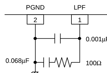
Figure 8.3 LPF External Circuit Connection Diagram
