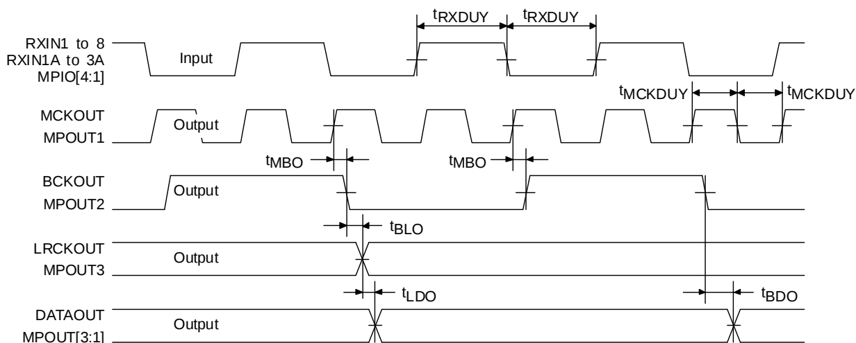
Figure 7.1 AC Characteristics 1
