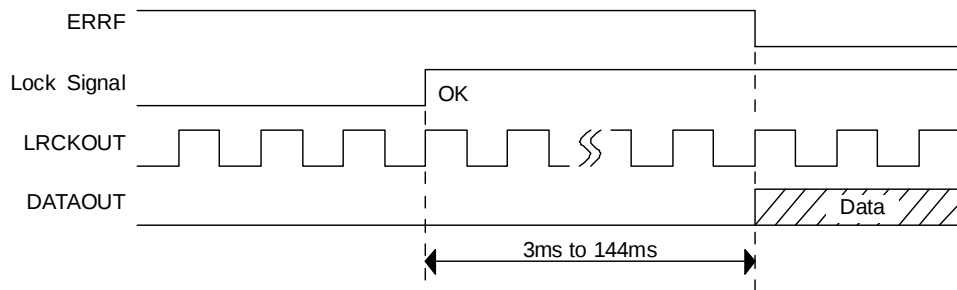
Figure 10.8 Data Processing When Data Demodulation Starts
