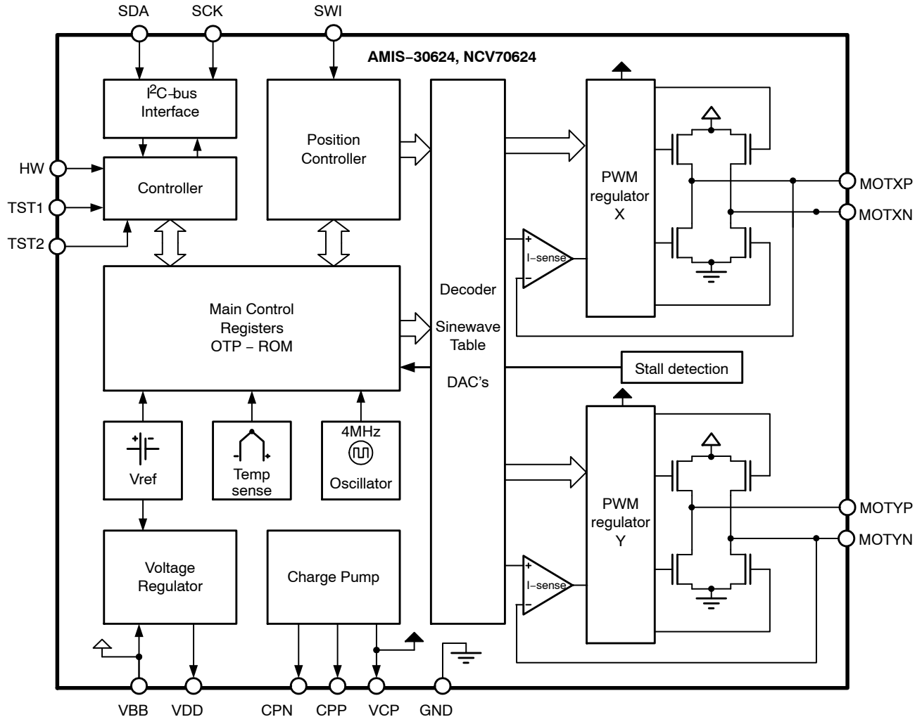
Figure 1. Block Diagram
