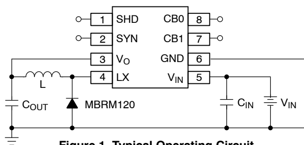
Figure 1. Typical Operating Circuit
