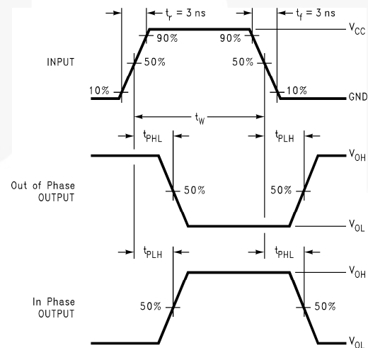
Figure 6. AC Waveforms
