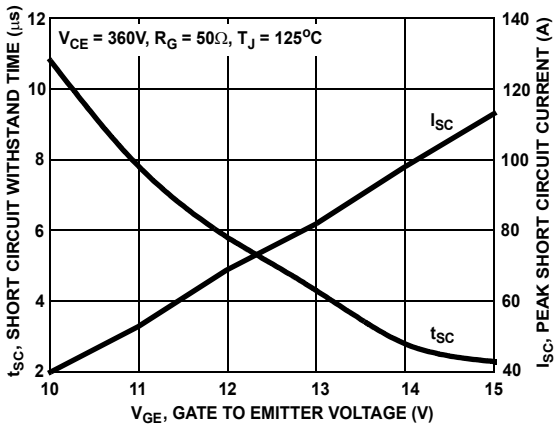
Figure 6. SHORT CIRCUIT WITHSTAND TIME
