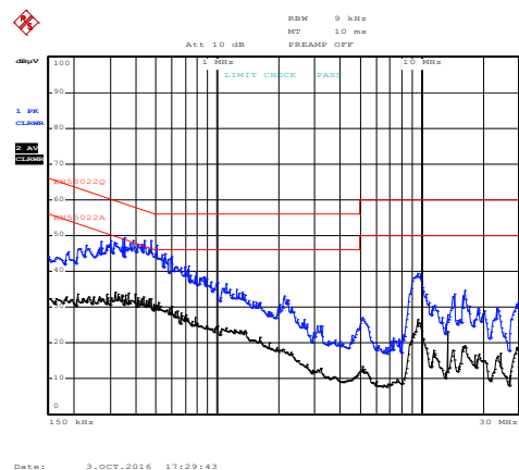
Figure 8. 120 V AC , 60 Hz, <N>.
