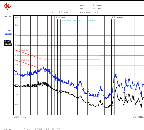
Figure 10. 220 V AC , 60 Hz, <N>.
