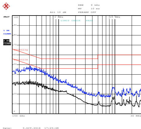
Figure 7. 120 V AC , 60 Hz, <L>.
