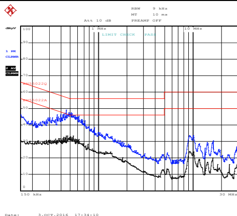
Figure 9. 220 V AC , 60 Hz, <L>.
