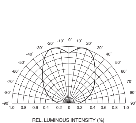
Fig. 4 Radiation Diagram
