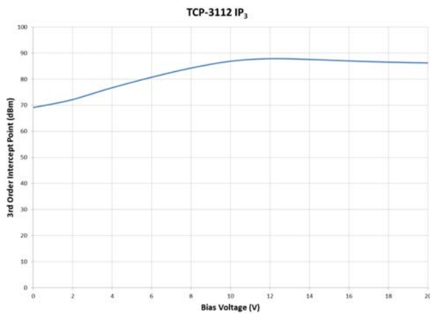
Figure 4. IP3*
