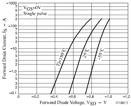
Figure 5. I_S - V_{SD}
