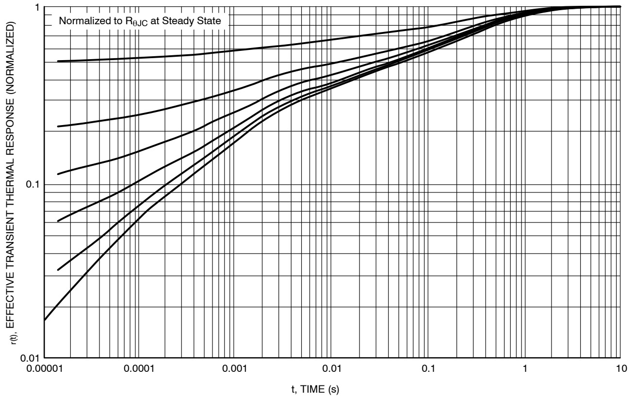
Figure 13. Thermal Response
