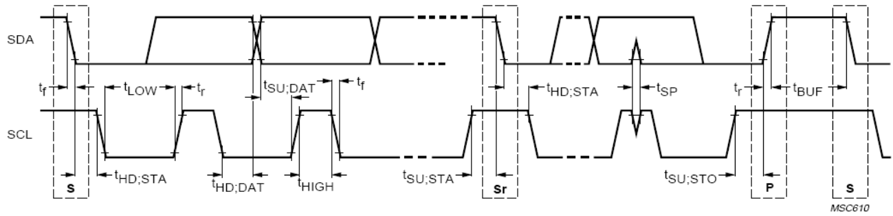
Figure 3. AC Characteristics
