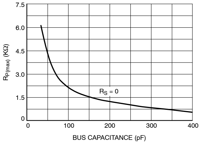
Figure 14. Maximum Value of R_P (in k\Omega ) as a function of Bus Capacitance (in pF)
