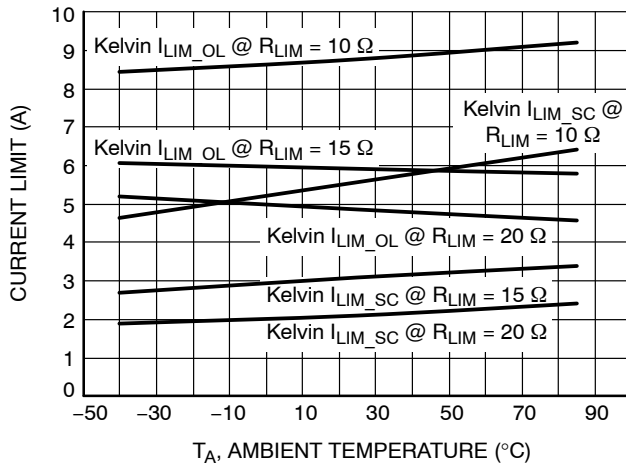
Figure 13. I_{LIM} vs. R_{LIM} over Ambient Temperature
