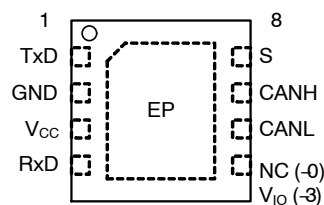
NCV7357D1x (Top View)
