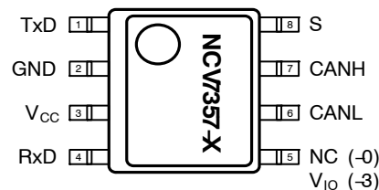
NCV7357MWx (Top View)
