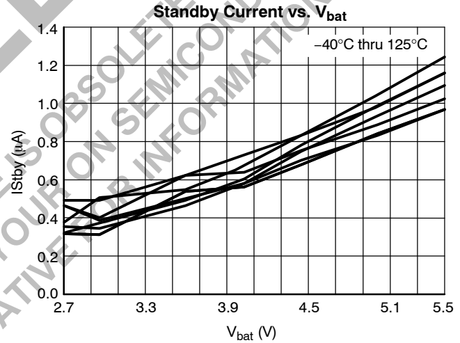
Figure 17. Standby Current
