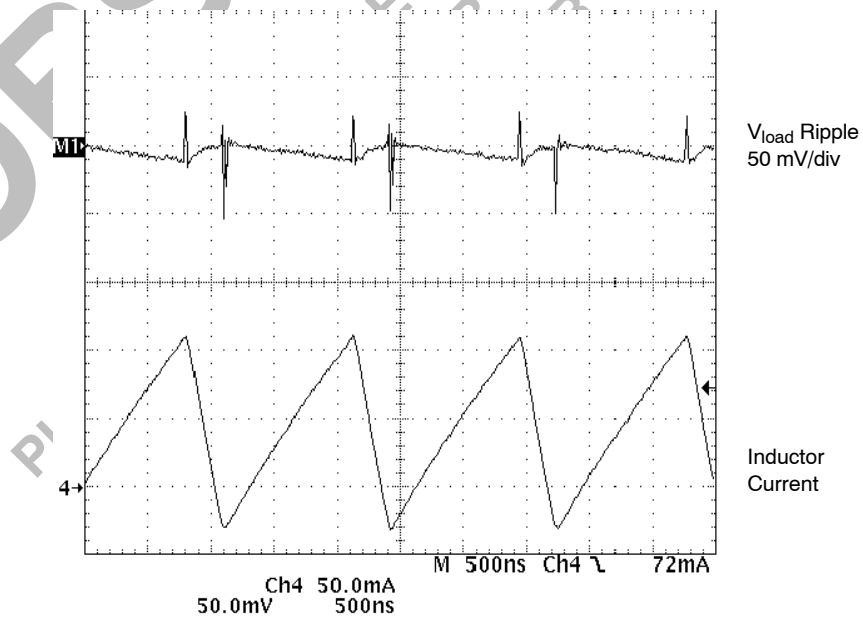
Figure 23. Typical Output Load Voltage Ripple
