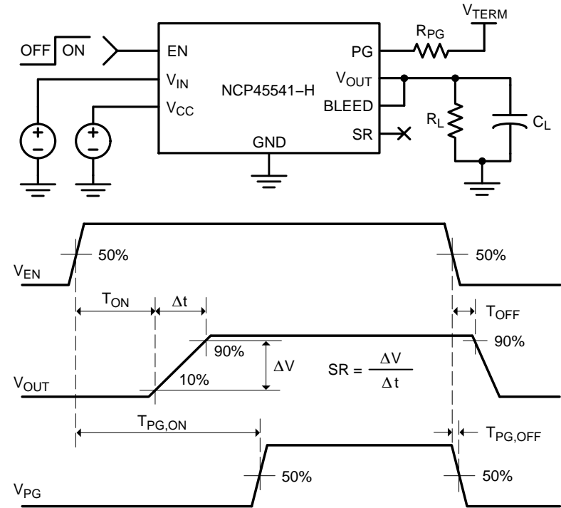
Figure 2. Switching Characteristics Test Circuit and Timing Diagrams
