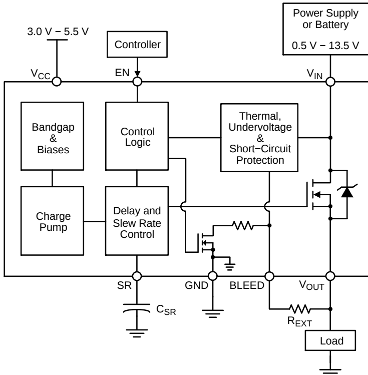
Figure 6. NCP45523 Typical Application Diagram – Load Switch
