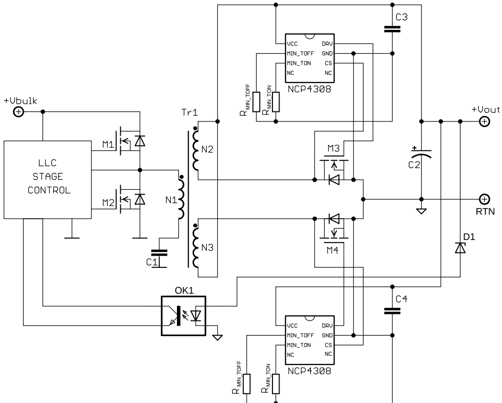
Figure 1. Typical Application Example – LLC Converter
