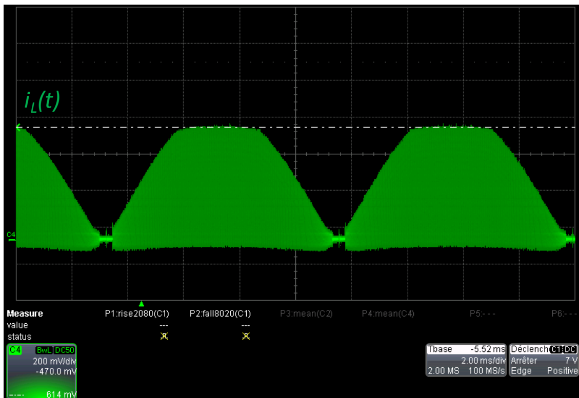
Figure 12. Inductor current showing OCP limitation @ V_{\text{mains}} = 90 \text{ V rms} ; F_{\text{mains}} = 60 \text{ Hz} ; I_{\text{load}} = 427 \text{ mA}
