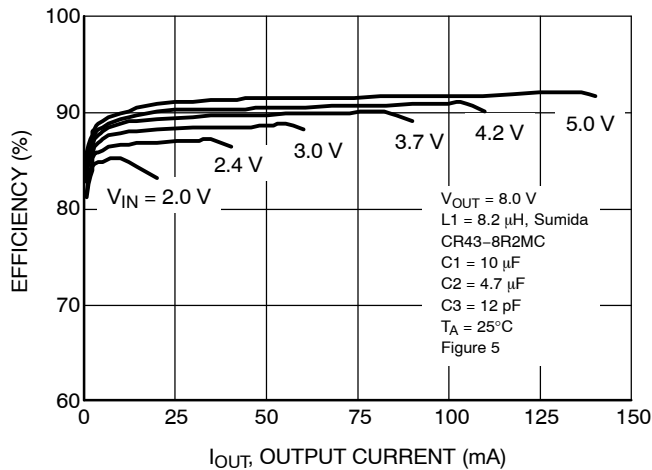
Figure 11. Efficiency versus Output Current ( V_{OUT} = 8\text{ V} , L = 8.2\text{ }\mu\text{H} )
