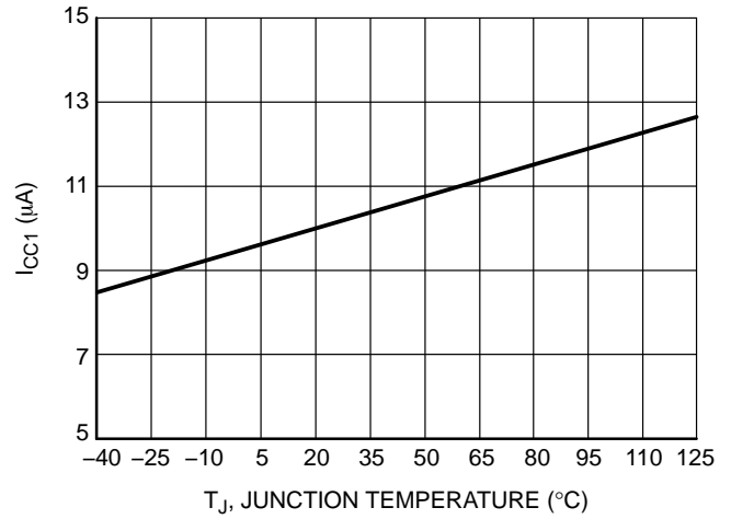
Figure 6. Internal Current Consumption before Start-Up, I_{CC1}
