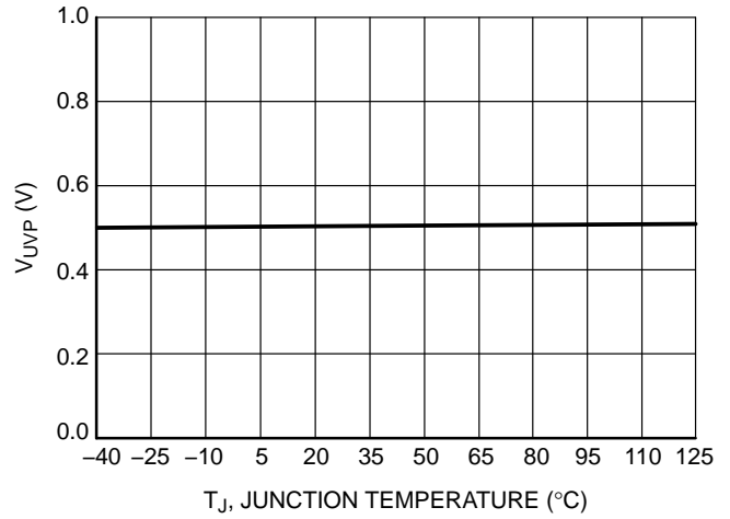
Figure 12. Undervoltage Detect Threshold, V_{UVP}
