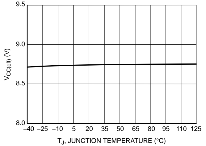
Figure 4. Minimum Operating Voltage, V_{CC(off)}
