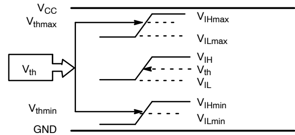
Figure 11. V_{th} Diagram
