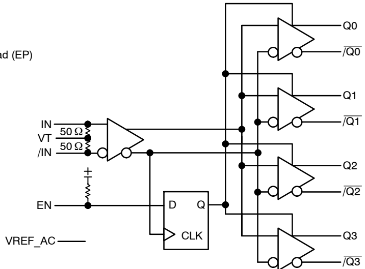
Figure 3. Logic Diagram
