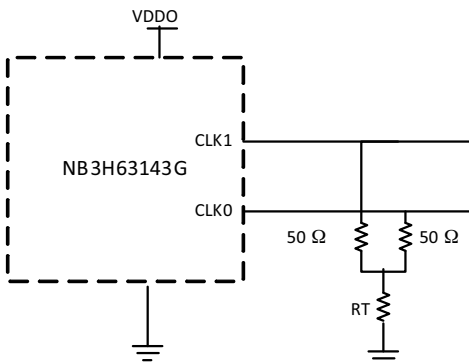
Figure 21. LVPECL Y-Termination
