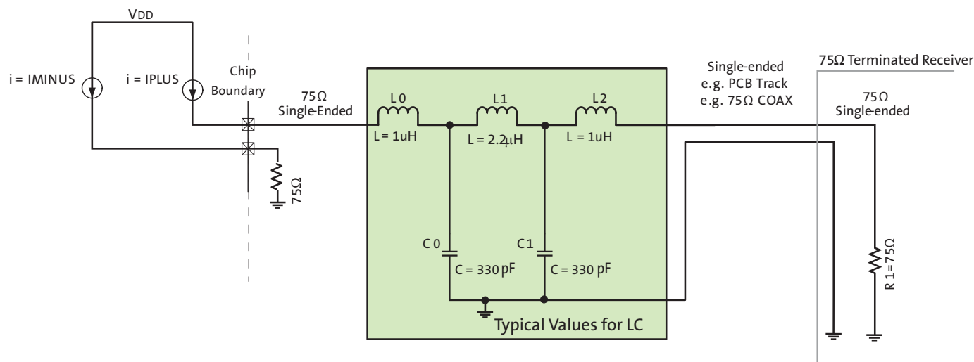
Figure 34: Single-Ended Termination
