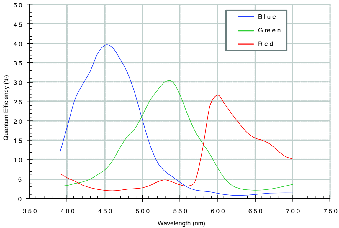
Figure 49. Quantum Efficiency
