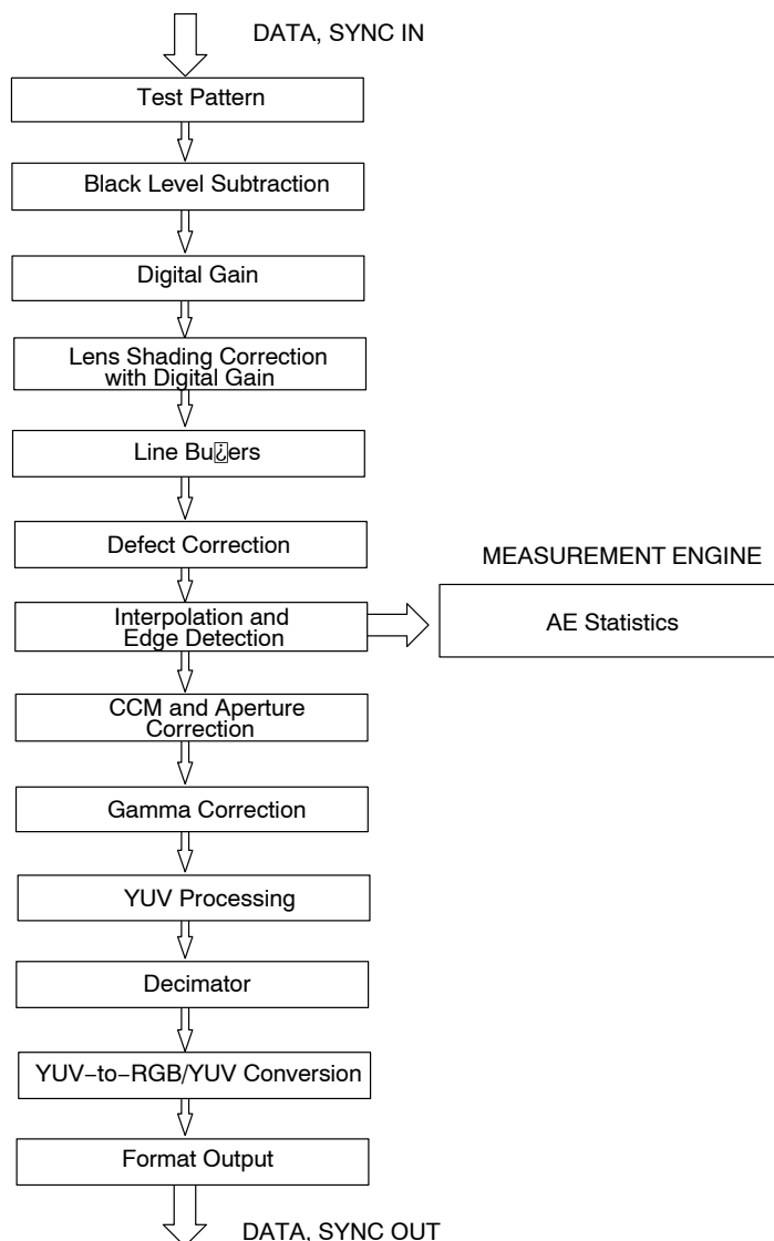
Figure 4. Color Pipeline
