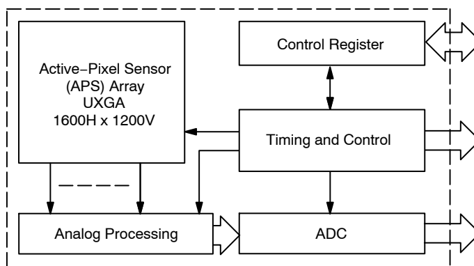
Figure 13. Sensor Core Block Diagram
