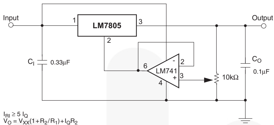
Figure 12. Adjustable Output Regulator (7 V to 30 V)
