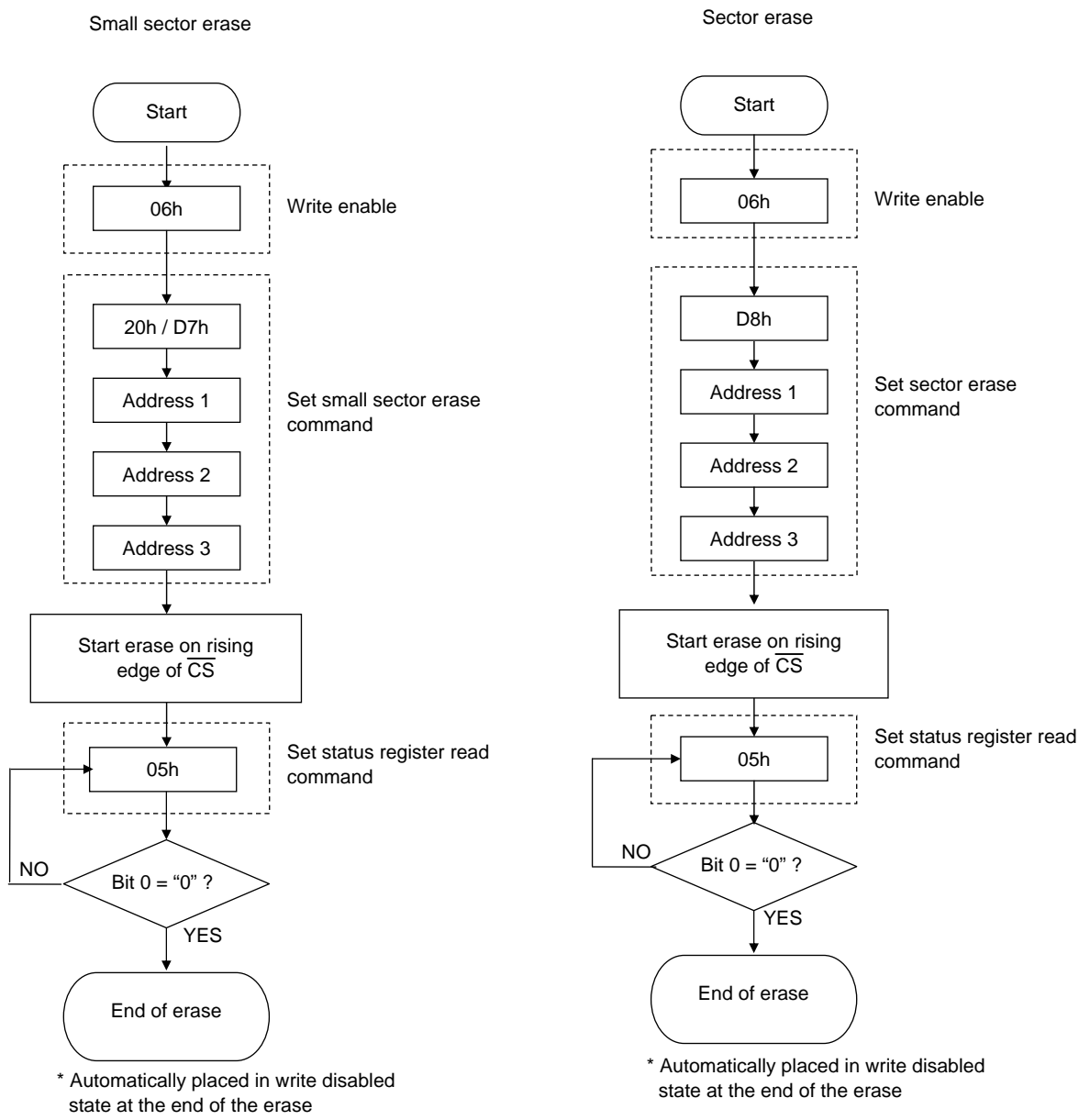
Figure 21 Erase Flowcharts
