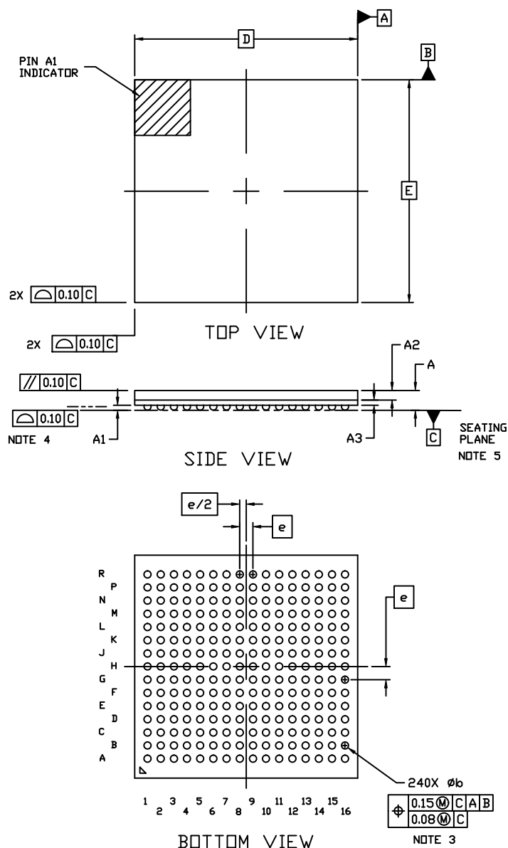
LFBGA240, 11x11 CASE 566EY ISSUE A
