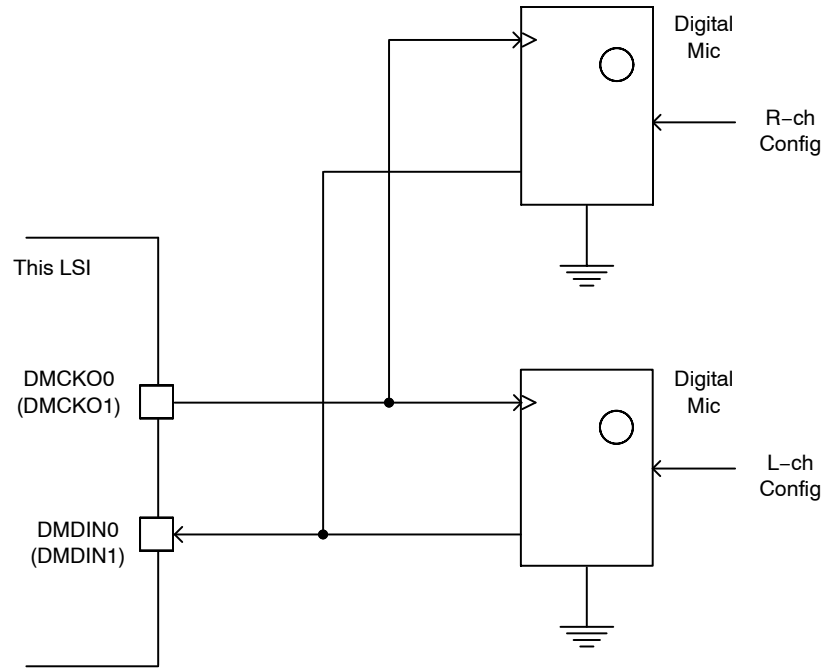
Figure 47. Digital Mic
