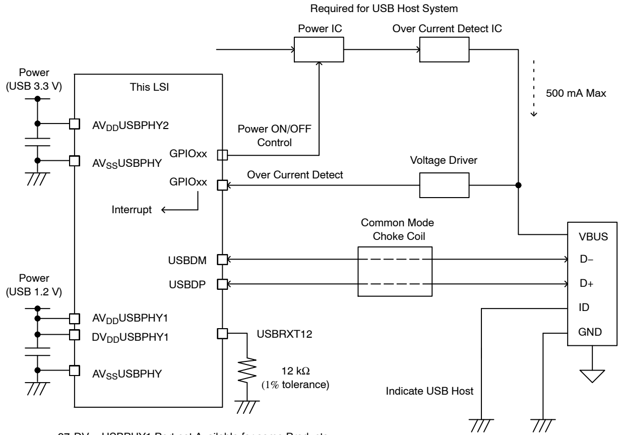
Figure 45. USB Host
