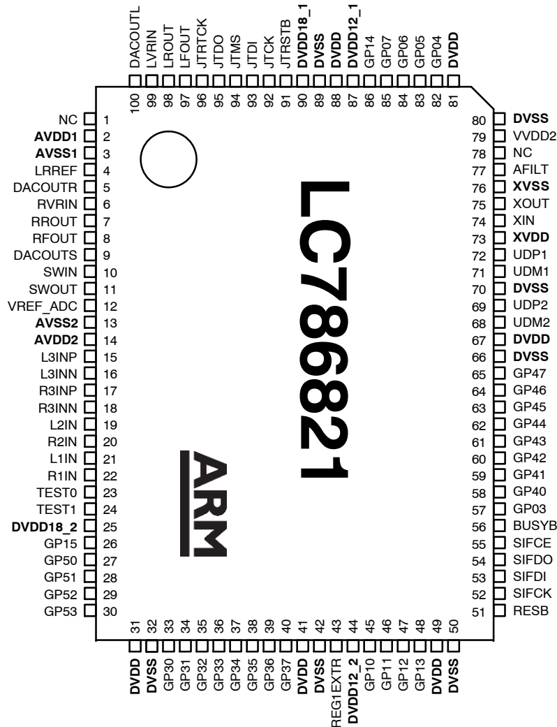
Figure 1. Pin Assignment
