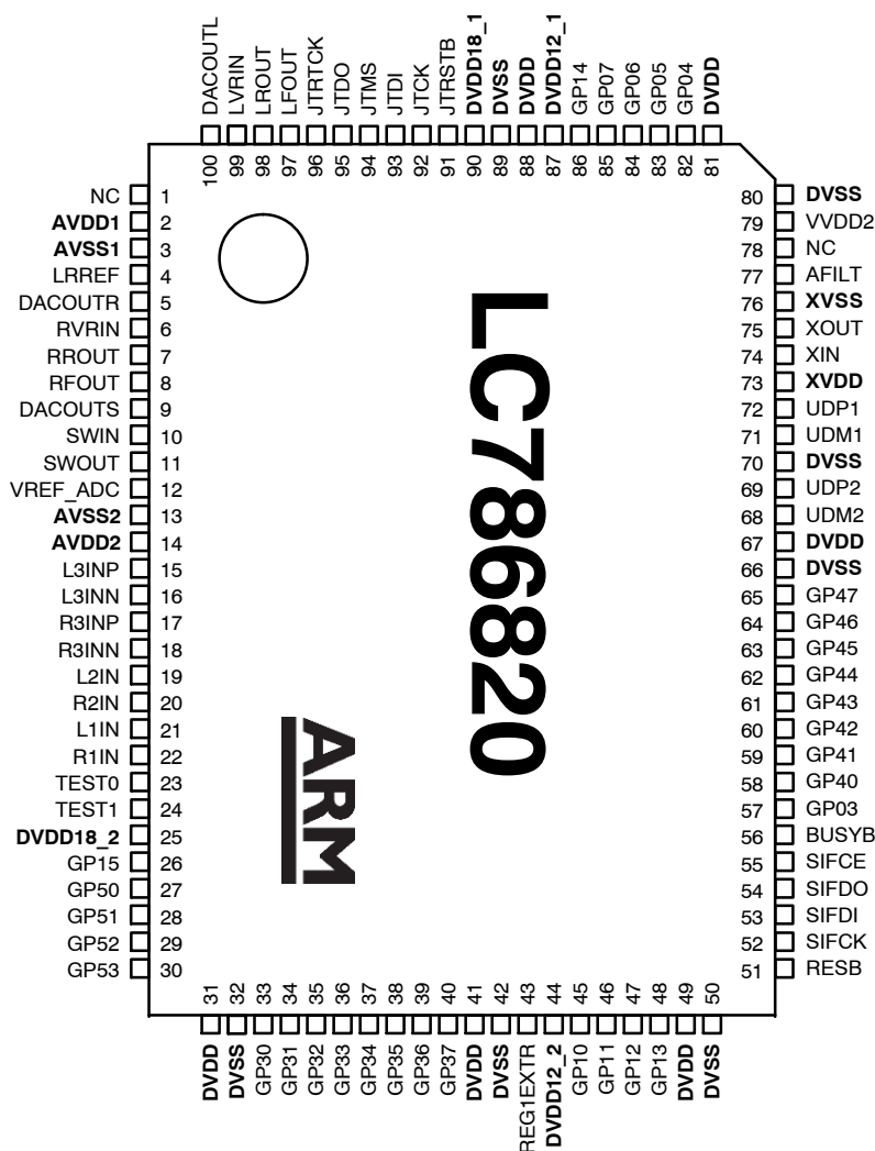
Figure 1. Pin Assignment
