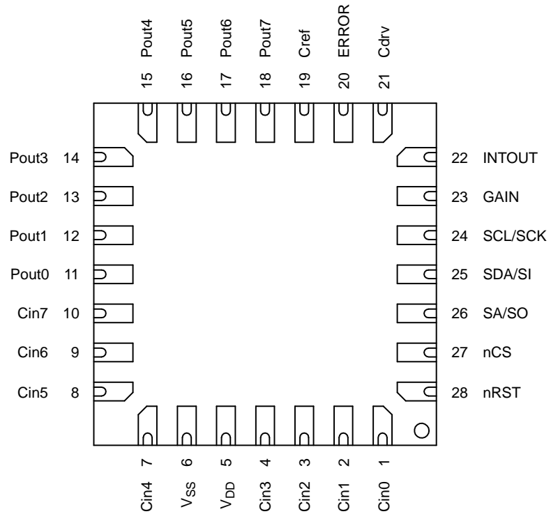
Figure 9. Pin Assignment
