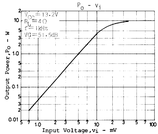
Figure 8. P_O - V_i
