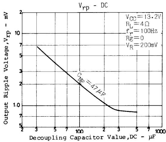
Figure 25. V_{rp} - DC
