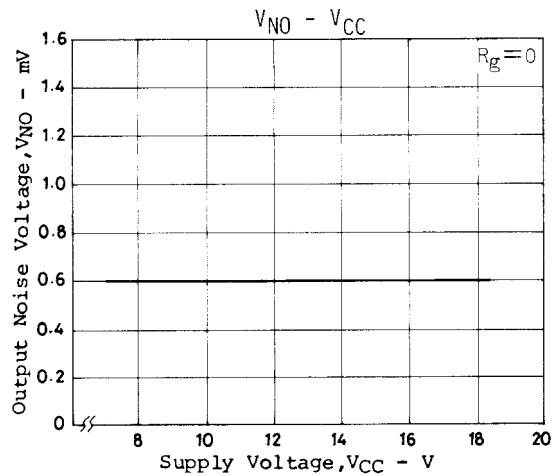
Figure 18. V_{NO} - V_{CC}
