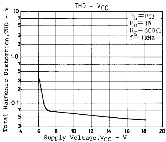
Figure 48. THD - V_{CC}
