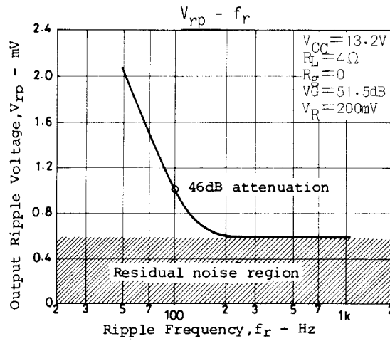
Figure 24. V_{rp} - f_r
