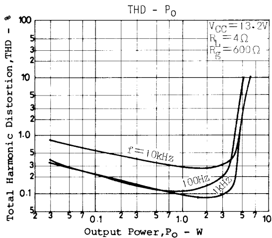
Figure 9. \text{THD} - P_O
