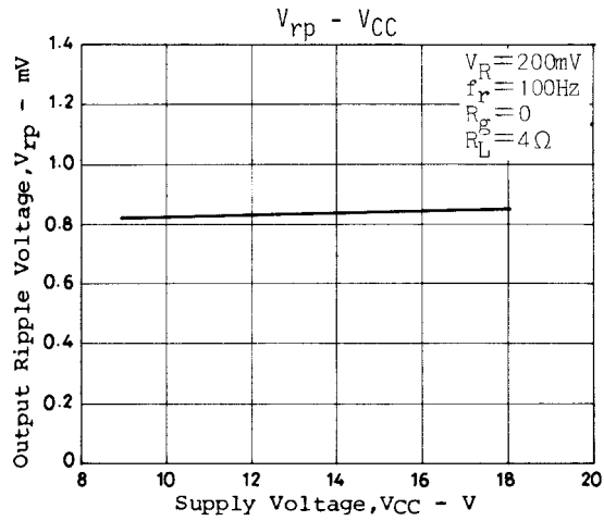
Figure 46. V_{rp} - V_{CC}
