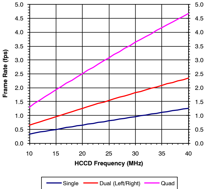
Figure 13. Frame Rates
