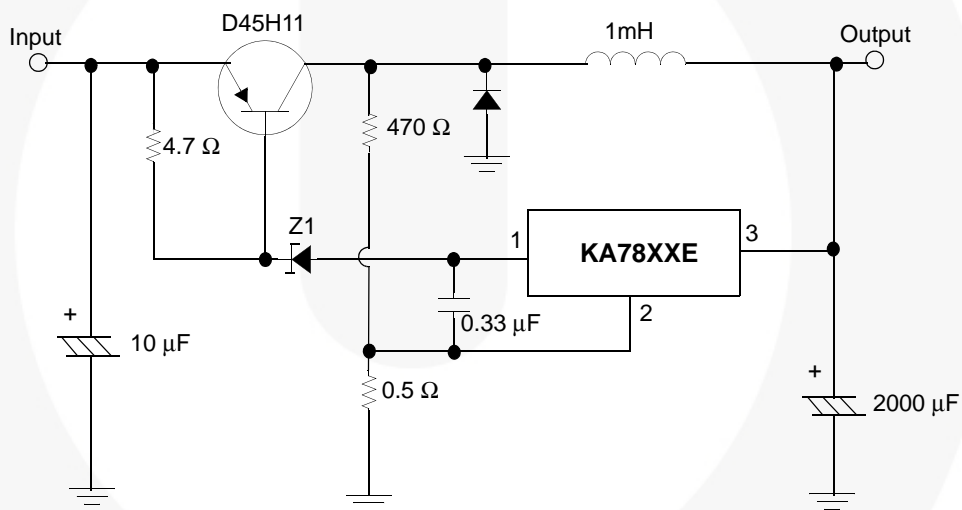
Figure 18. Switching Regulator
