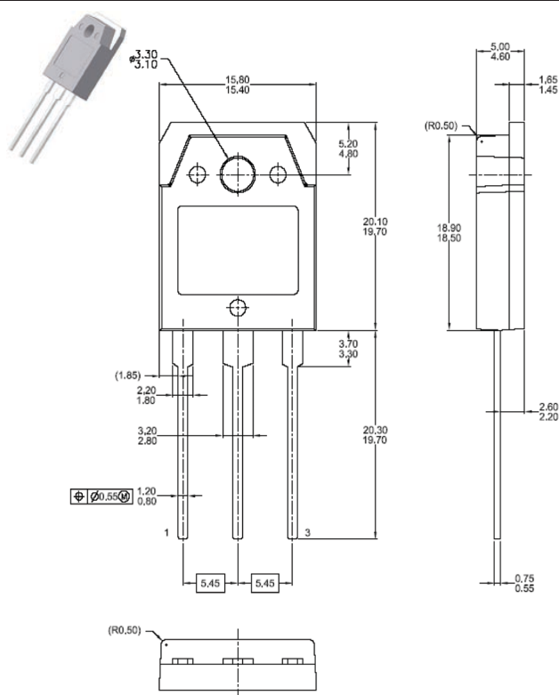
TO-3PN
