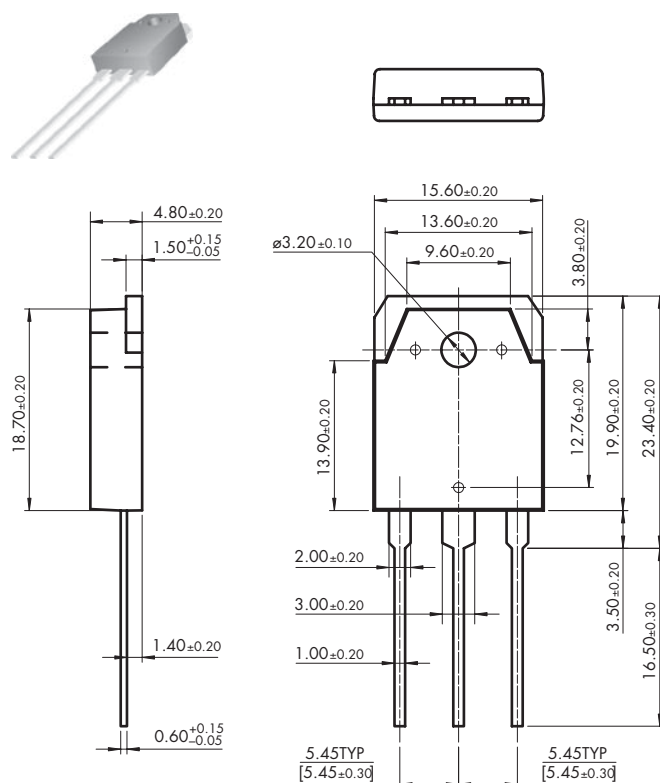
TO-3PN
