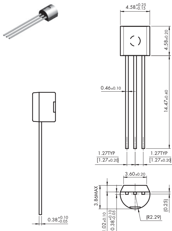
TO-92
