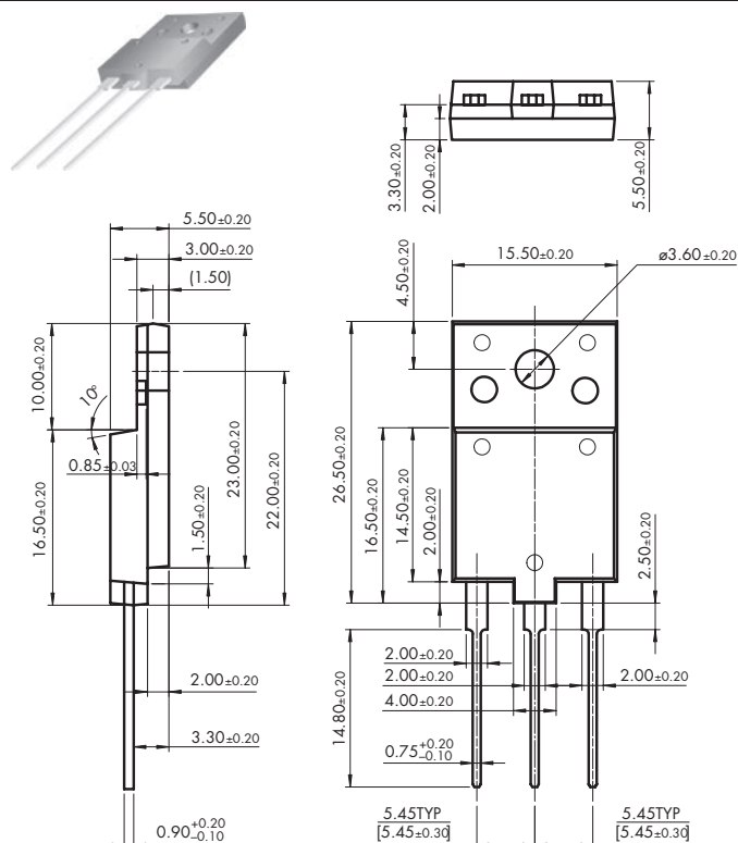
TO-3PF
