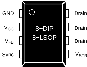
Figure 3. Pin Configuration (Top View)
