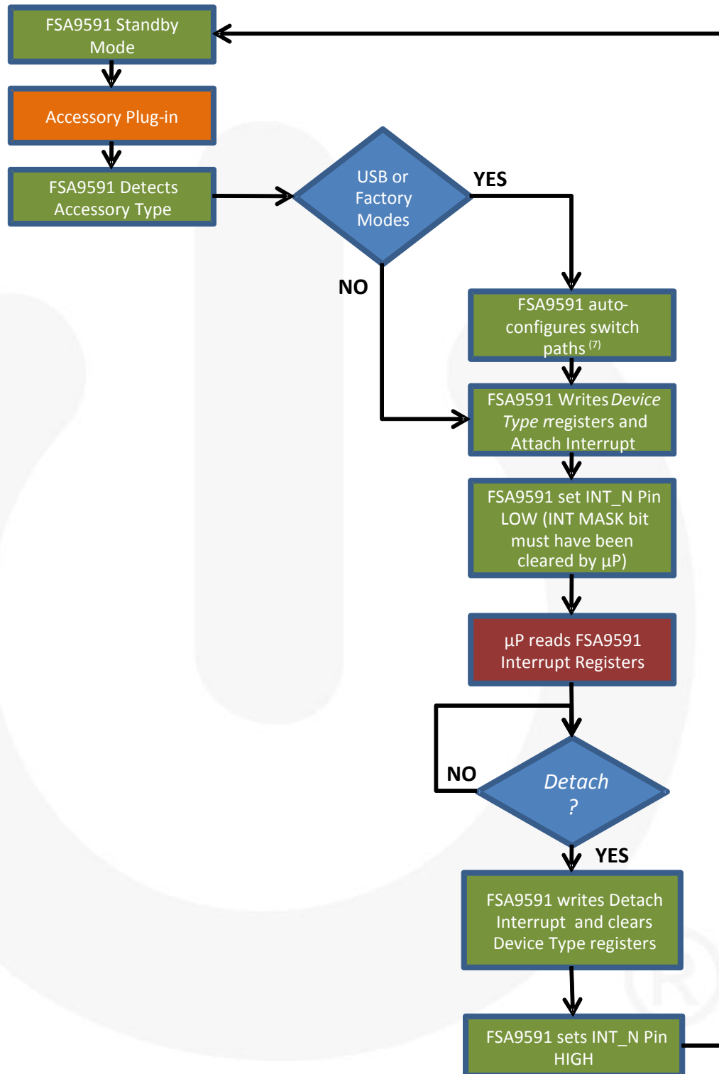
Figure 7. Factory Cable Detection
