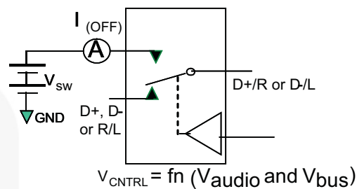
Figure 14. Off Leakage
