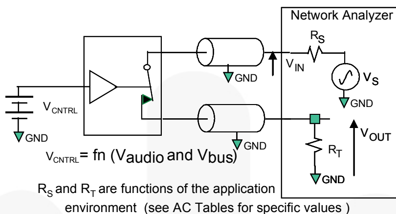
Figure 22. USB Bandwidth
