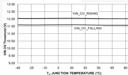
Figure 20. V IN_VOVL0 vs. Temperature
