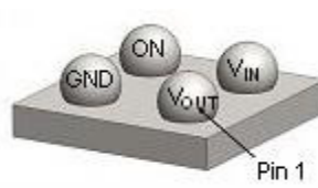
Figure 4. 1 x 1 mm WLCSP Bumps Facing Up
