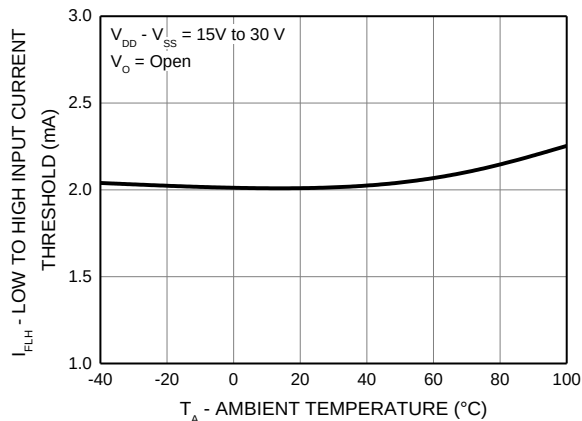
Figure 10. Low to High Input Current Threshold vs. Ambient Temperature
